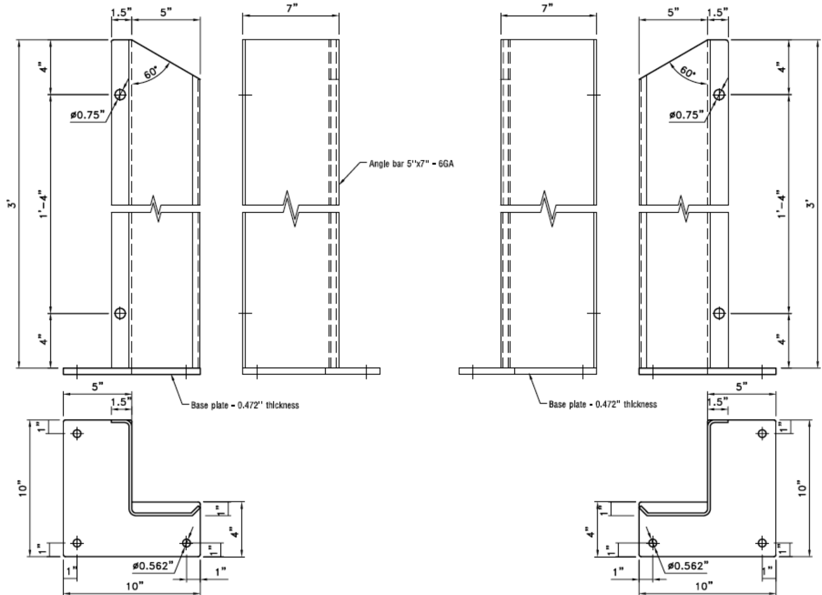
OVERHEAD DOOR TRACK GUARD 5"x7" - 36" LEFT
