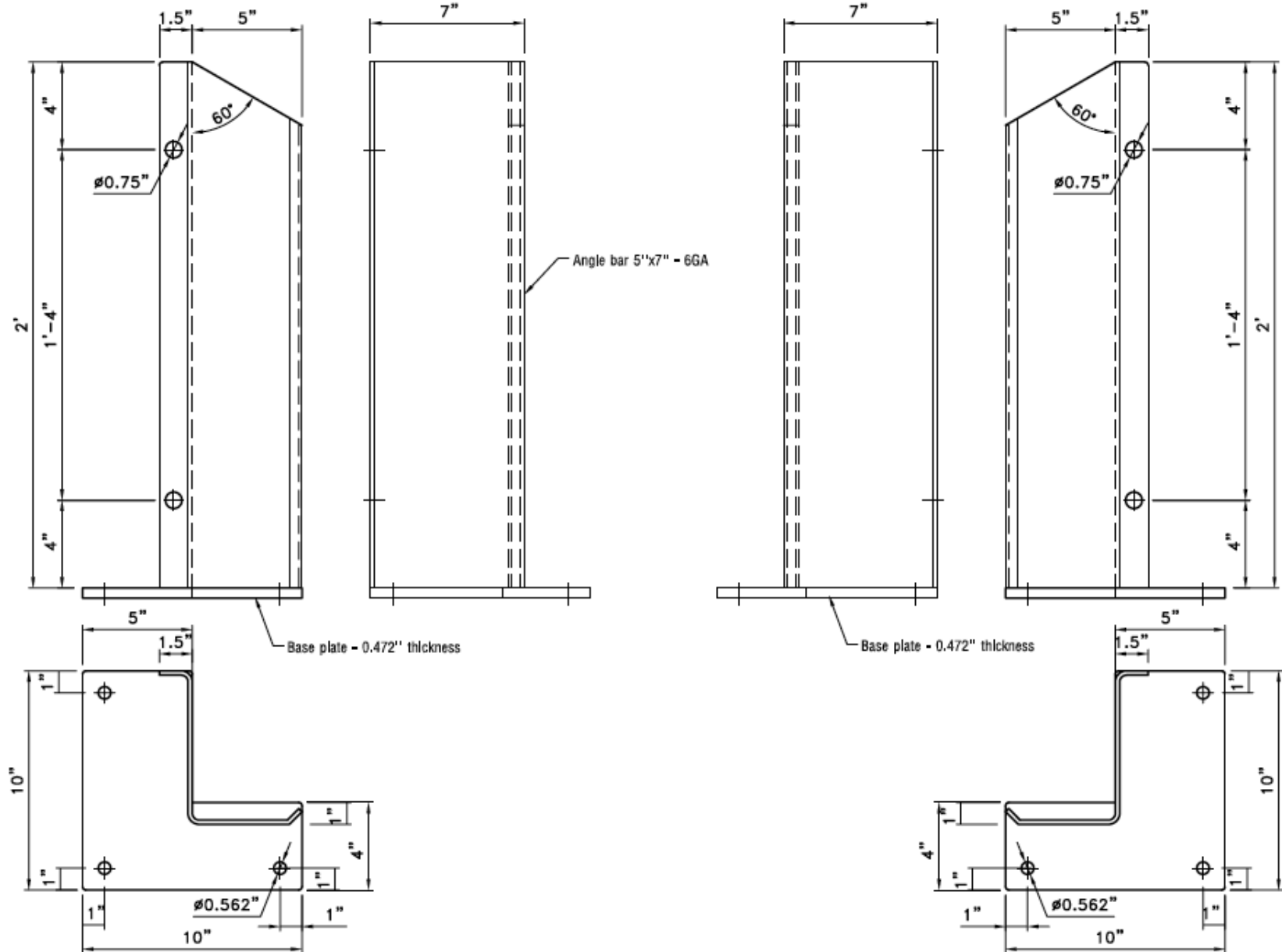
OVERHEAD DOOR TRACK GUARD 5"x7"- 24" LEFT
